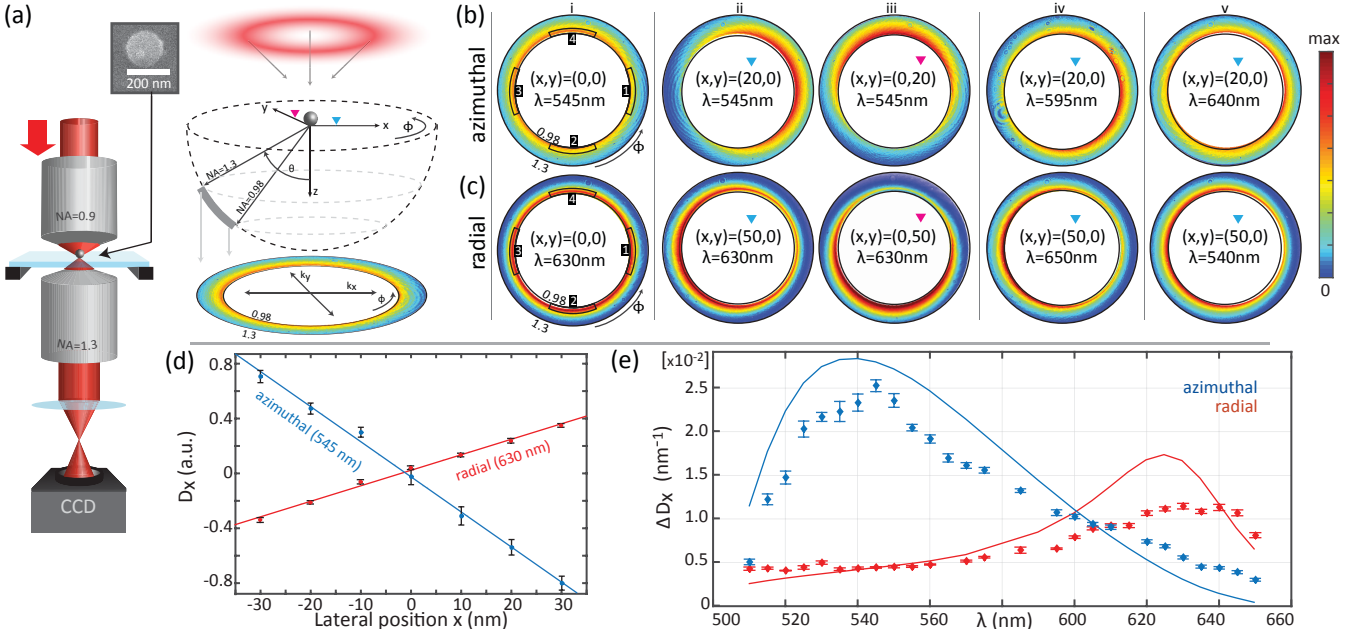
FIG. 3. Experimental implementation. (a) A collimated input beam (radially or azimuthally polarized) is tightly focused using a microscope objective of numerical aperture (NA) of 0.9 onto a silicon nanoantenna sitting on a glass substrate (SEM image in inset), which can be precisely positioned by a piezo-stage. The forward scattered light is collected using an oil-immersion type microscope objective of NA = 1.3. The back-focal plane (BFP) is imaged onto a CCD camera. (b-c) Exemplary BFP images showing symmetric scattering for an on-axis position (i), and transverse Kerker directionality for off-axis positions (ii-v). The strength of directional scattering strongly depends on the wavelength as shown in (ii-v) with maximum directionality observed at \lambda_{\text{azim}} = 545 nm (b. ii-iii) and \lambda_{\text{rad}} = 630 nm (c. ii-iii). (d) Plot of the measured directivity D_x versus the antenna's x -position for \lambda_{\text{rad}} = 630 nm (in red) and \lambda_{\text{azim}} = 545 nm (in blue). (e) The slope of these curves ( \Delta D_x ) is plotted for all wavelengths along with the numerically calculated results for comparison (radial and azimuthal polarization in red and blue).
