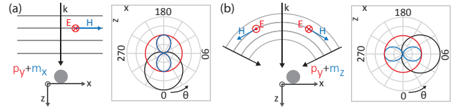
FIG. 1. Kerker scattering and Huygens’ dipole. (a) Zero backscattering. A y -polarized plane wave with \mathbf{k} = k_z \hat{\mathbf{e}}_z excites transverse electric and magnetic dipoles p_y and m_x of equal amplitudes and phases, resulting in a Huygens’ dipole and zero backscattering. (Inset) Polar plot of the resulting total far-field intensity of the scattered light (black) and the individual emission patterns of p_y (red) and m_x (blue) in the meridional xz -plane. (b) Directional scattering perpendicular to the propagation direction of the beam (transverse Kerker scattering). A tightly focussed azimuthally polarized beam propagating along the z -axis can induce longitudinal magnetic m_z and transverse electric p_y dipoles, resulting in transverse Kerker scattering [inset similar to (a)].
