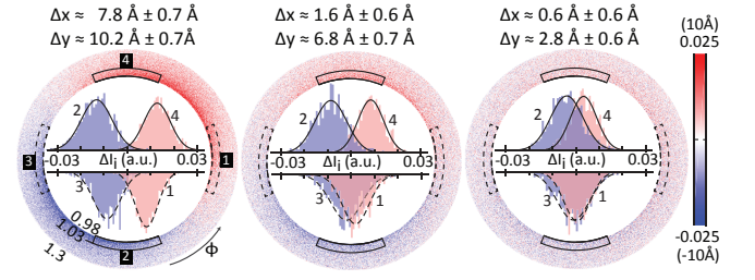
FIG. 4. Differential BFP images for relative displacements of less than 1 nm for an azimuthally polarized excitation beam with \lambda_{\text{azim}} = 545 nm ( \Delta D_x \approx \Delta D_y \approx 0.025 \text{ nm}^{-1} ). In each BFP image, \Delta I_j values from the outlined regions are used to plot the histograms shown in the centers; dash-outlined regions ( j = 1, 3 ) correspond to \Delta x and solid-outlined regions ( j = 2, 4 ) to \Delta y . Gaussian fits to the \Delta I_j distributions (histogram) are used to estimate the relative displacements (peak-to-peak) and the precision of estimation (standard error of the mean). The Gaussian peaks are clearly distinguishable for a relative displacement down to 3 Å, with precision of 0.6 Å.
